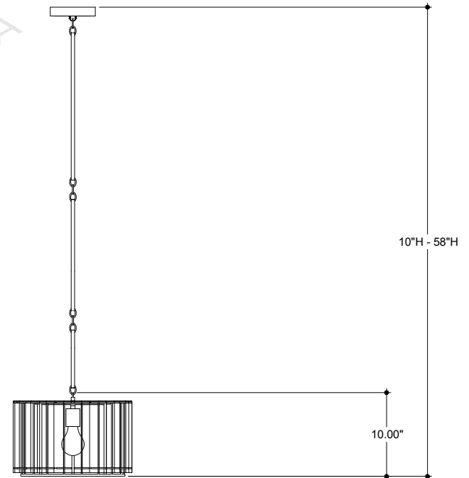
LEFT VIEW
