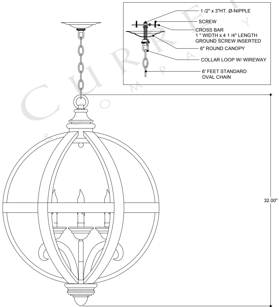
FRONT VIEW
