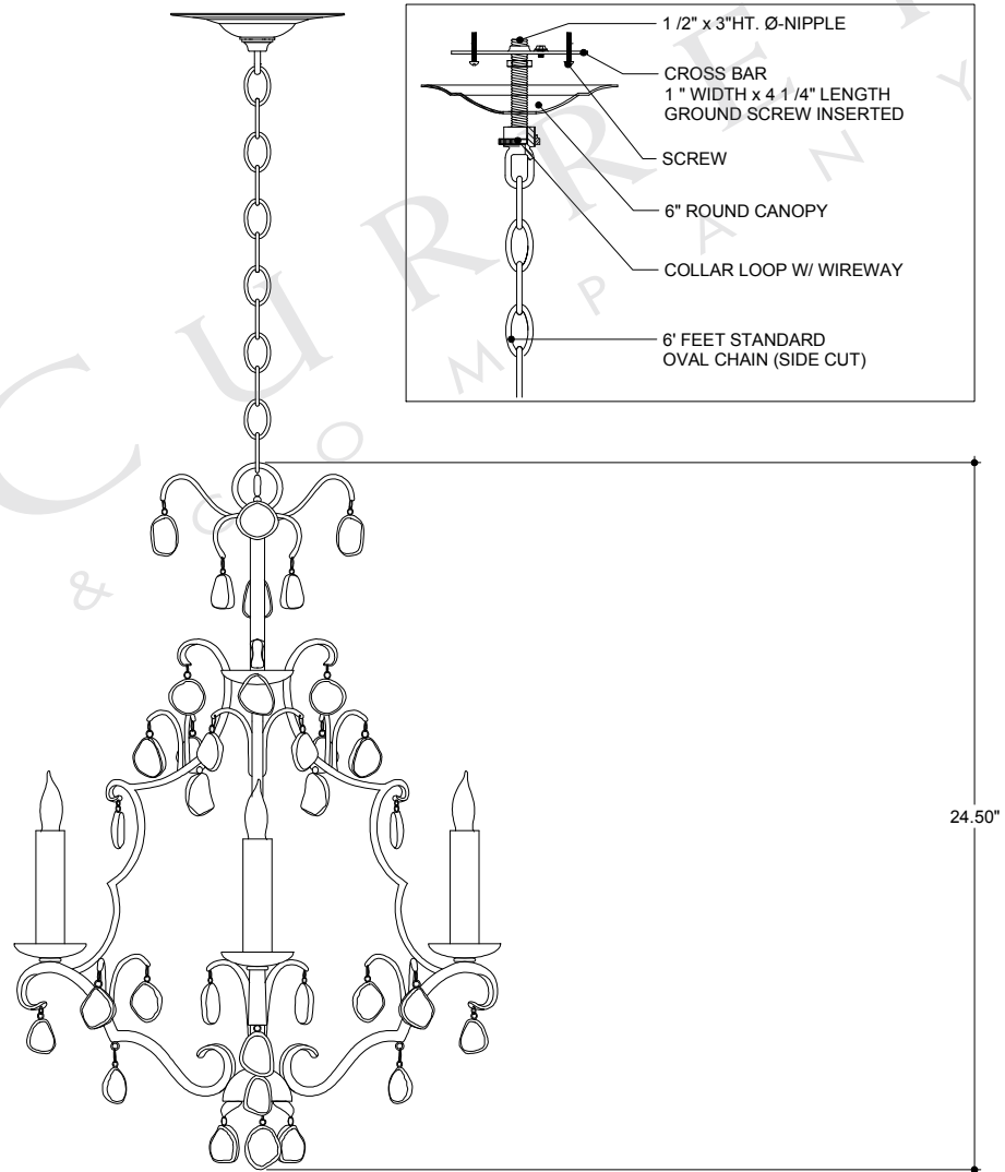
FRONT VIEW
