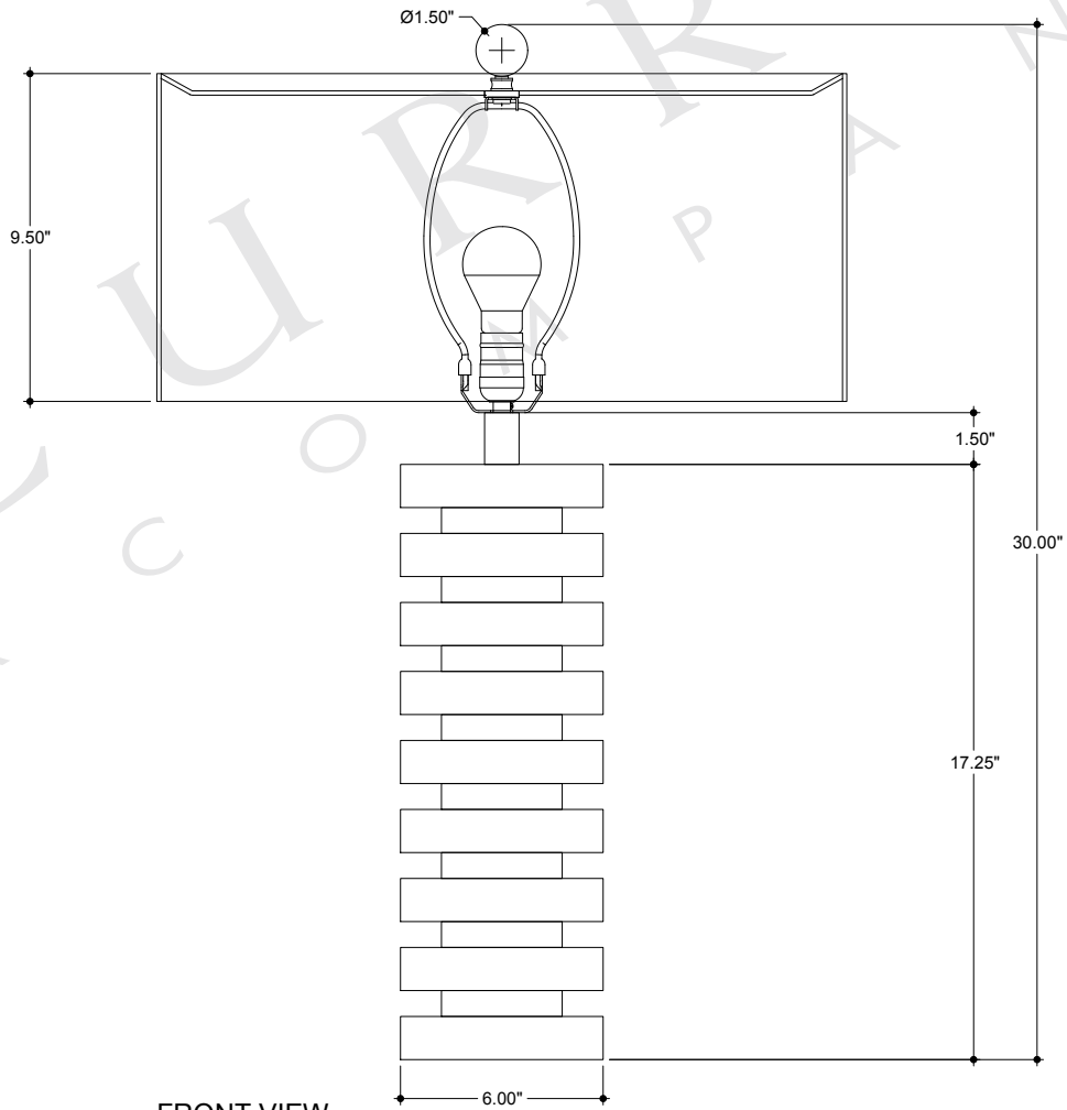
FRONT VIEW
